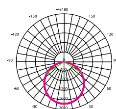
50W 600x1200 Panel Light PL-CCT60120
