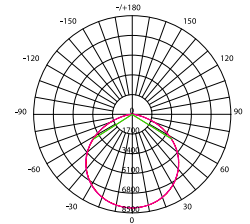
200W UFO High Bay PL-UF-200W
