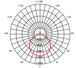
150W UFO High Bay PL-UF-150W
